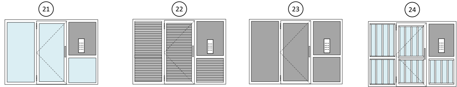
Single Leaf Door and Two Side screens with cut out for door entry
